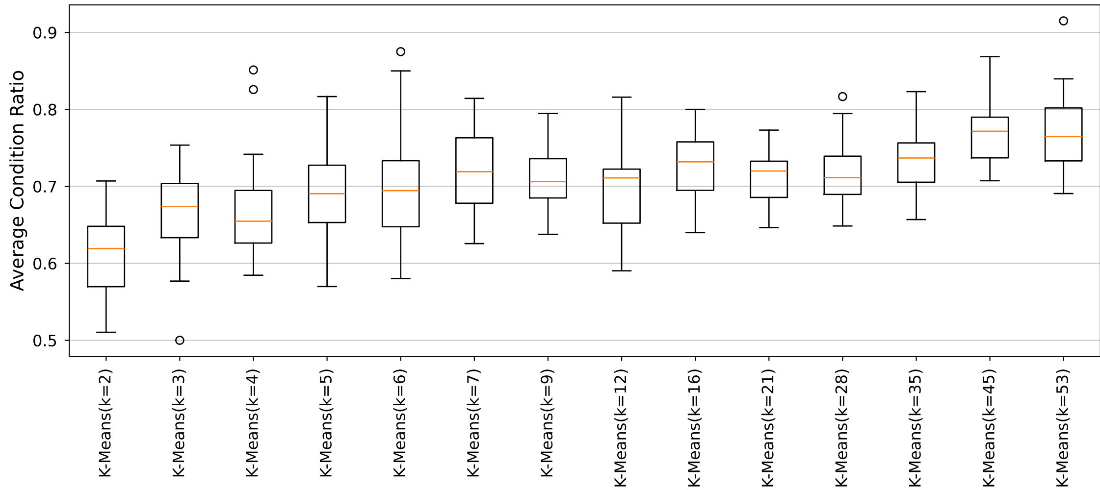
YARA Rules Average Condition Ratio Distribution (Cluster3_Size53 dataset)
